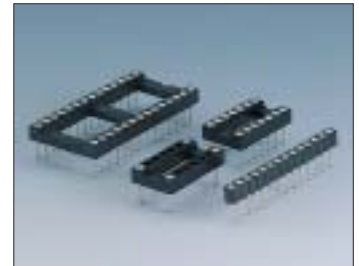
2.54mm(.100") 3310 SERIES ROUND PIN I.C. SOCKET 3312 SERIES ROUND PIN SIP SOCKET 3313 SERIES OSCILLATOR SOCKET
