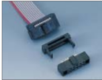
1.27mmx1.27mm(.050"x0.50") 6920 SERIES I.D.C. SOCKET
