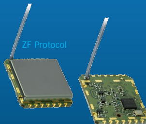
RF Stamp Receiver AFZE-1005, 868 MHz (IFM) AFZE-5004, 915 MHz (IFM) AFZE-1007, 868 MHz (DCM) AFZE-5007, 915 MHz (DCM)
